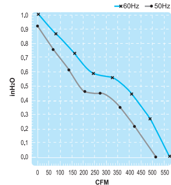
(Axial Fan)
