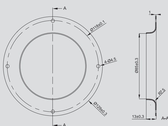
133A (For UF133APA)
