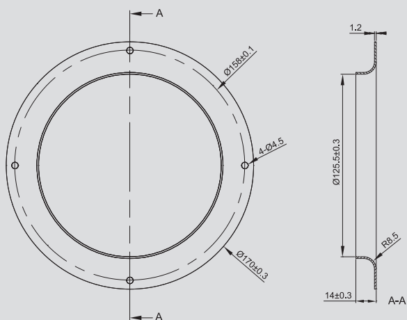
190A (For UF190APA, UF180APA and UF175AMA)
