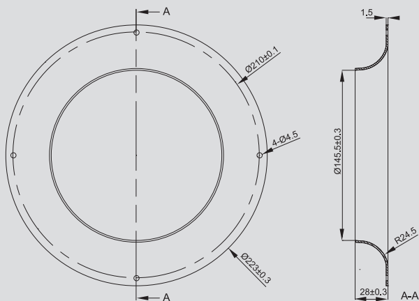
225A (For UF225 Series)
